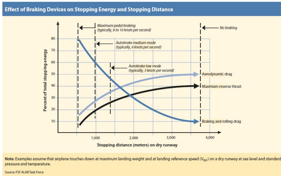
FIGURE 2. BRAKING DEVICES ON STOPPING ENERGY AND STOPPING DISTANCE
