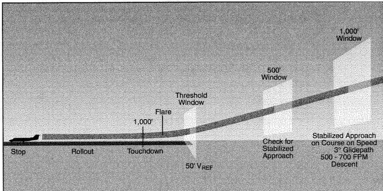
FIGURE 1-1. STABILIZED APPROACH
