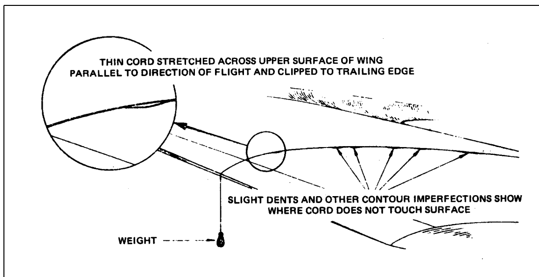
Figure 3 Checking Contours
