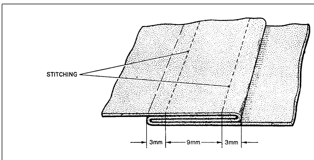
Figure 1 Balloon Seam
