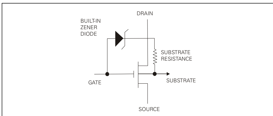
Figure 2 A Typical Protected MOS Device
