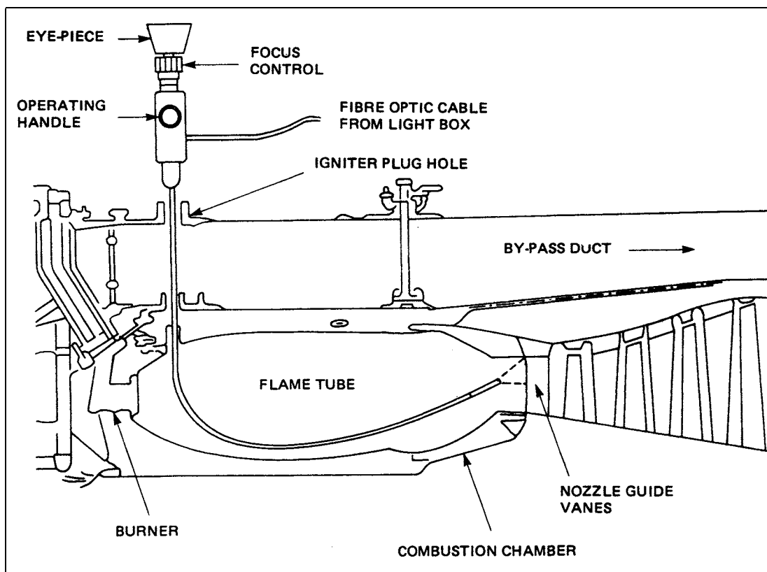
Figure 1 Flexible Endoscope Inspection Equipment
