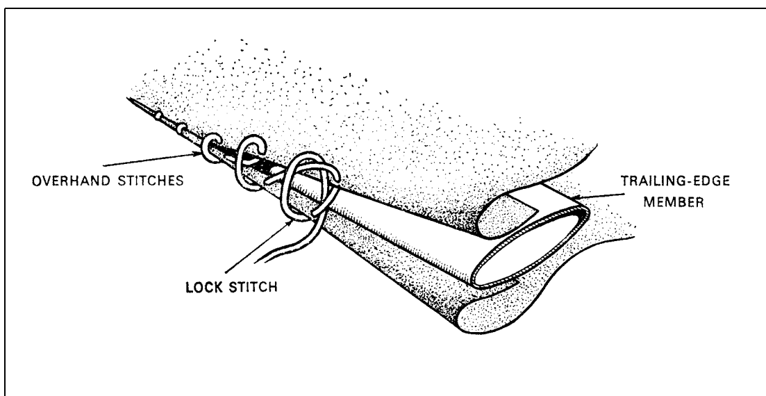
Figure 3 Overhand Stitch
