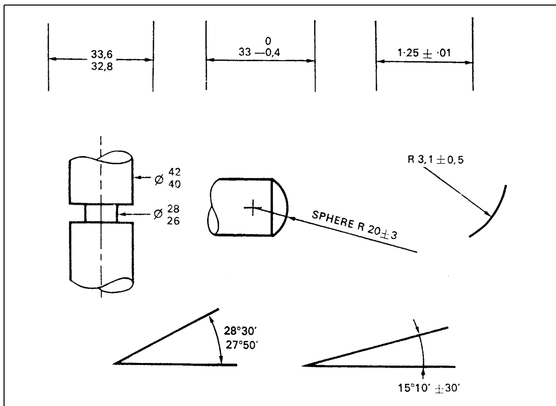
Figure 14 Dimensional Tolerances
