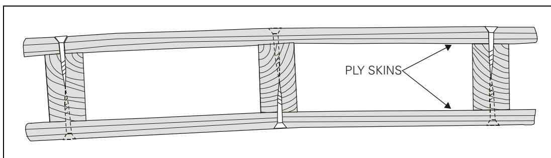
Figure 1 Double Skin Structure
