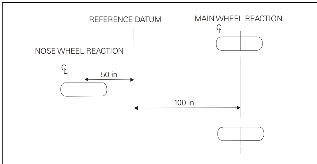
Figure 10 Centre-of-Gravity Relative to the Reference Datum
