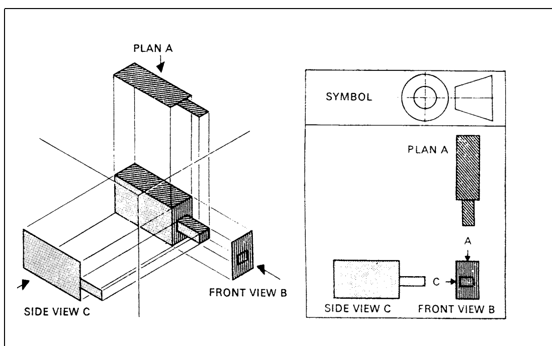
Figure 2 Third-angle Projection
