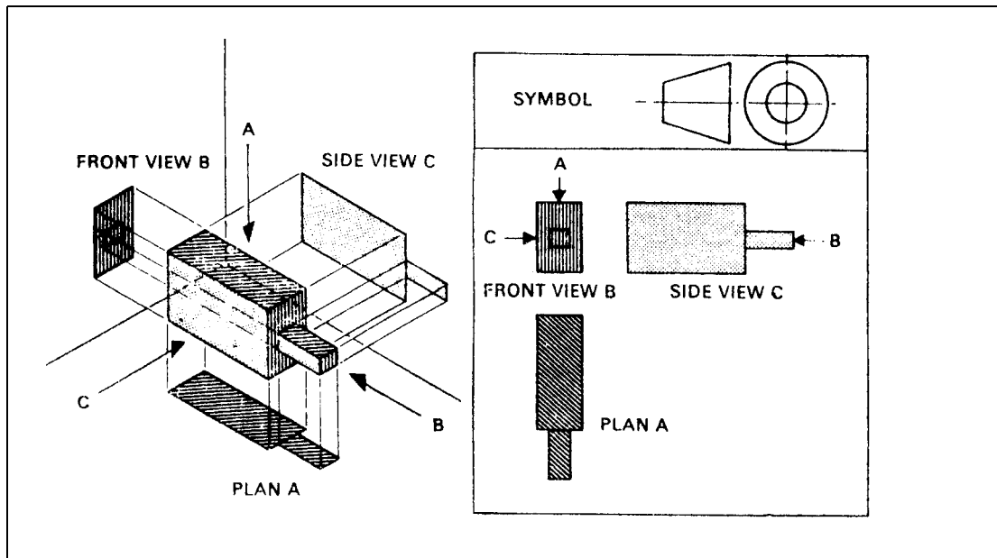
Figure 3 First-angle Projection
