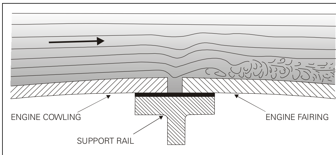
Figure 1 Drag Due to Gap in Cowlings
