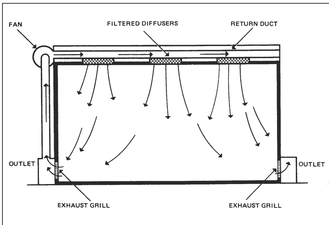
Figure 1 Conventional Flow System
