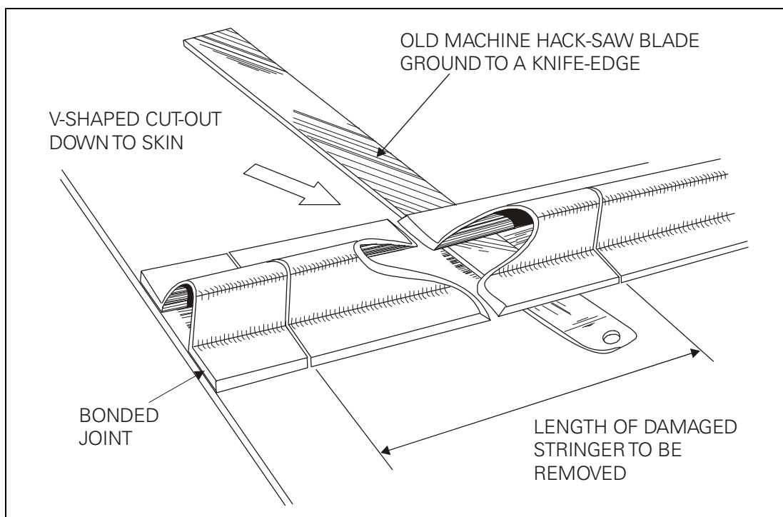
Figure 1 Removal of Bonded Component
