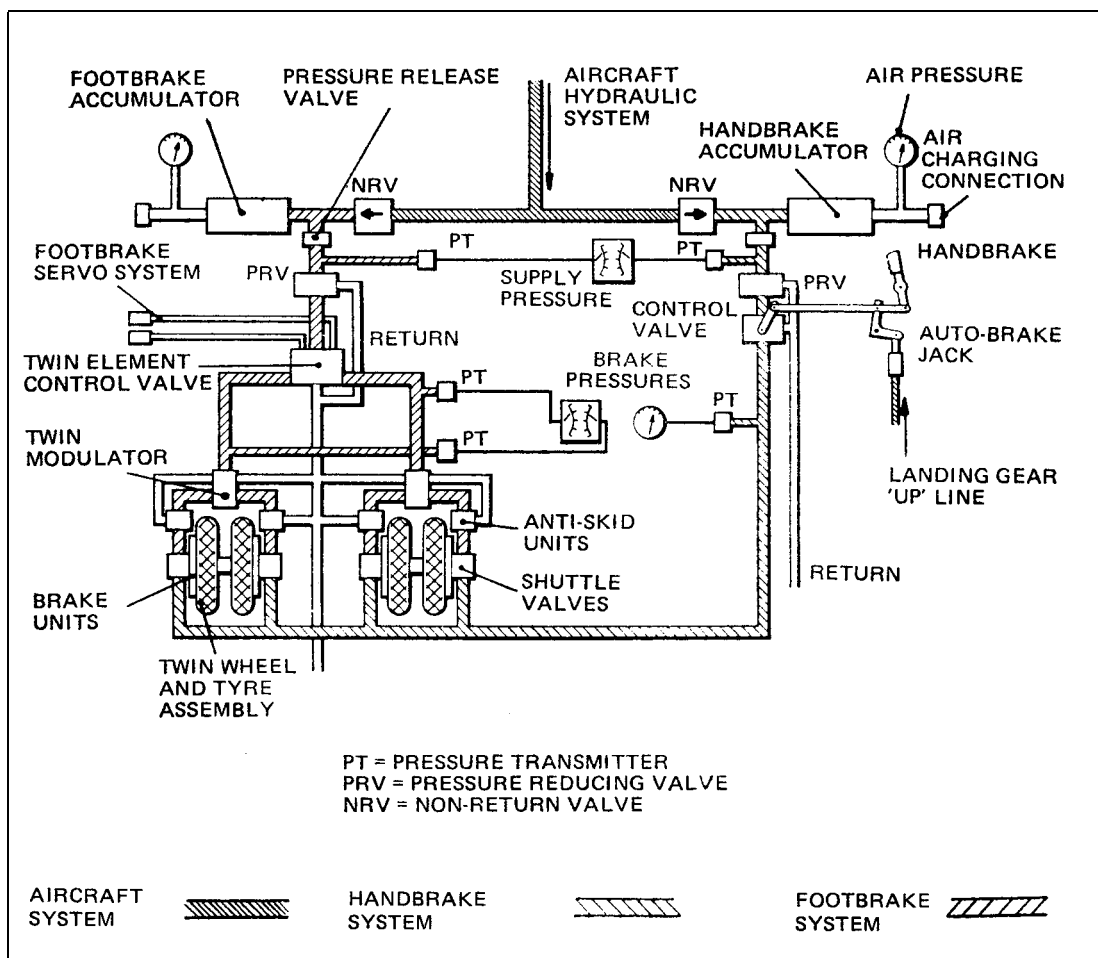
Figure 7 Simple High-pressure Brake System
