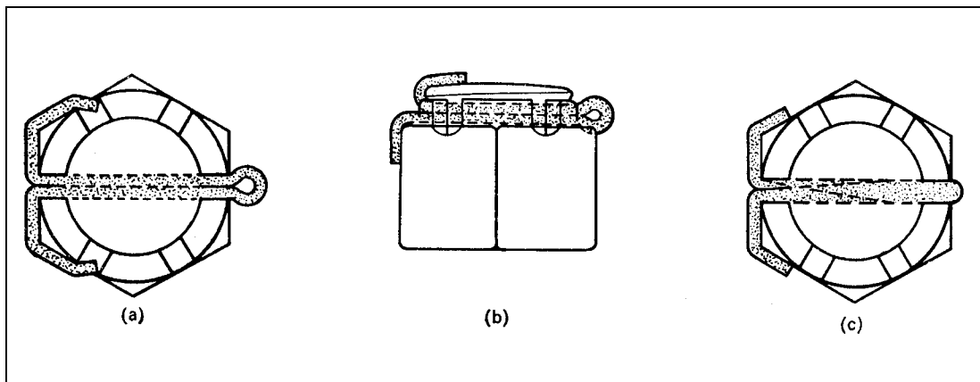
Figure 1 Split Pinning
