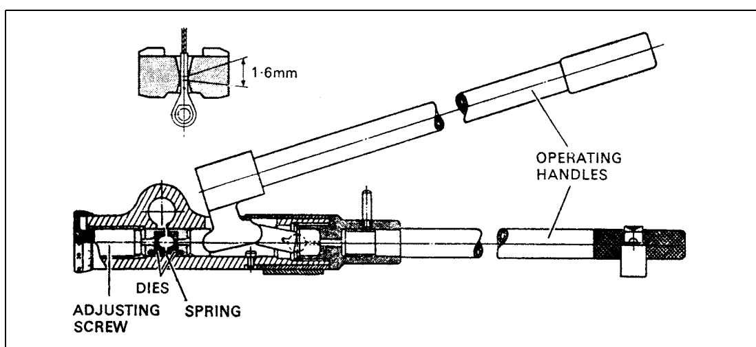
Figure 2 Portable Swaging Machine
