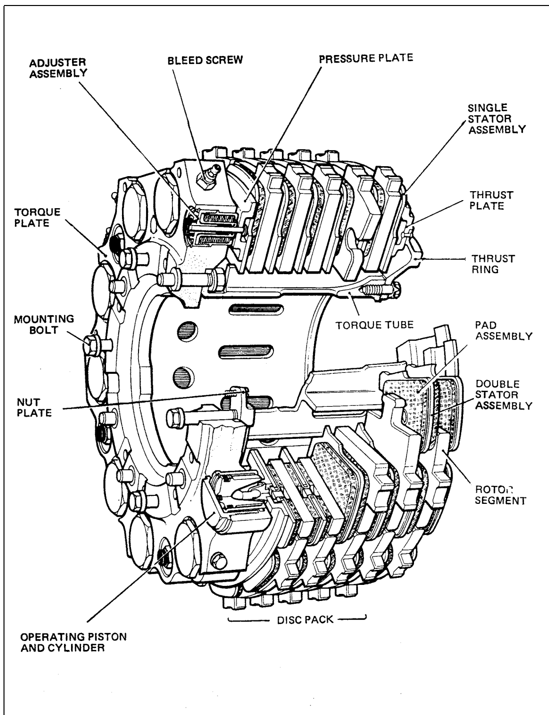
Figure 4 Multi-disc Brake
