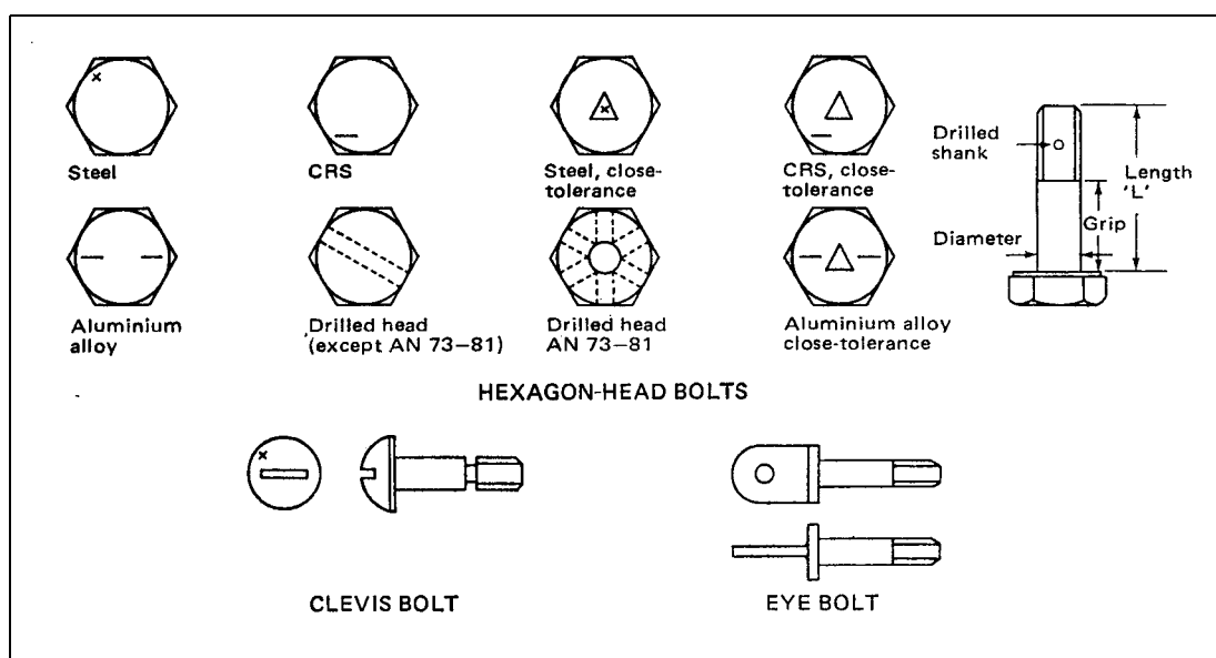
Figure 1 Early Series AN Bolts
