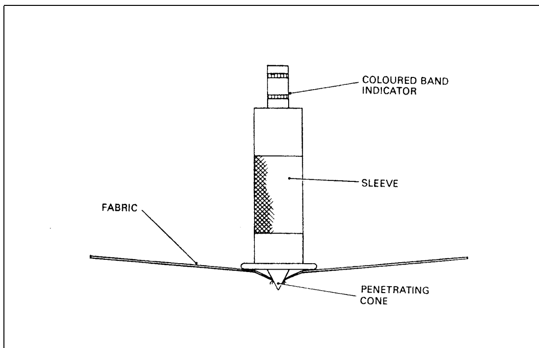
Figure 14 Fabric Tester
