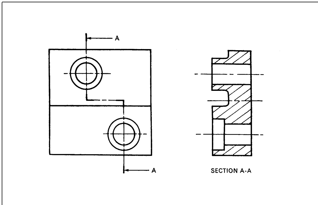
Figure 6 Staggered Section
