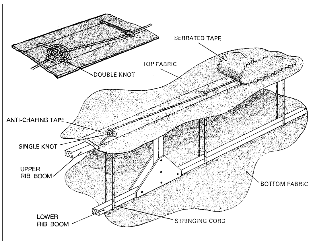
Figure 4 Typical Stringing
