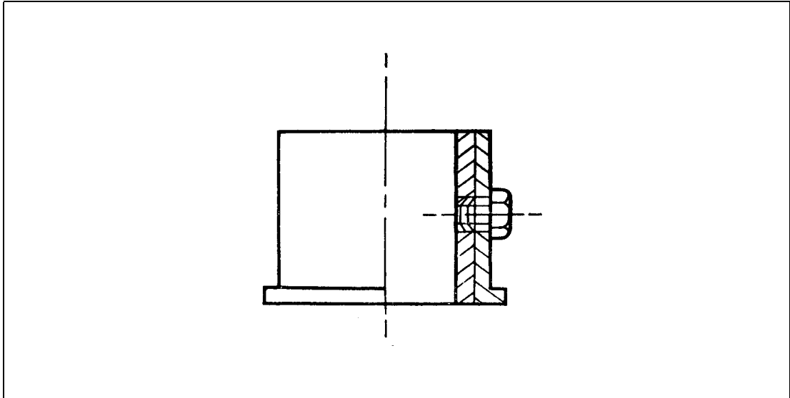
Figure 5 Half Section
