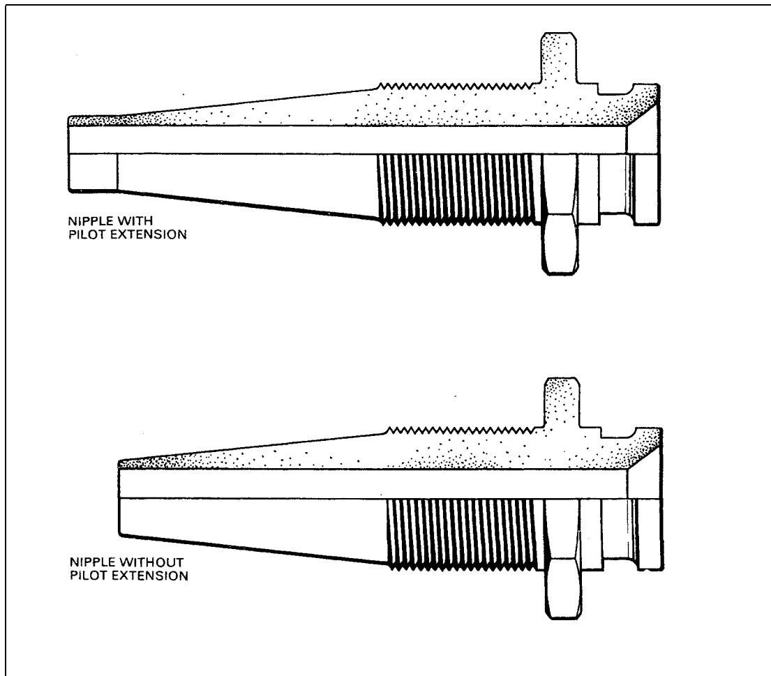
Figure 7 Nipple Characteristics
