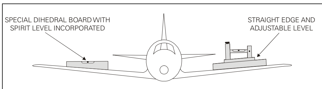
Figure 3 Checking Dihedral
