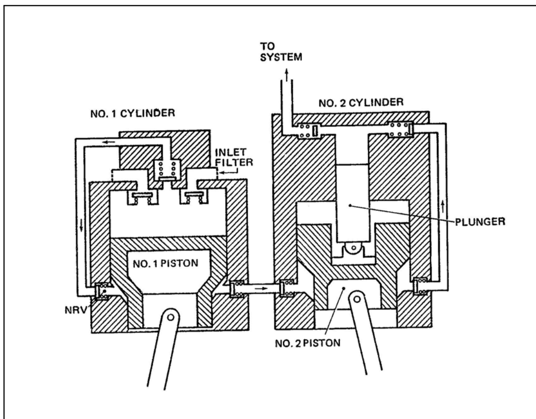
Figure 2 Air Compressor
