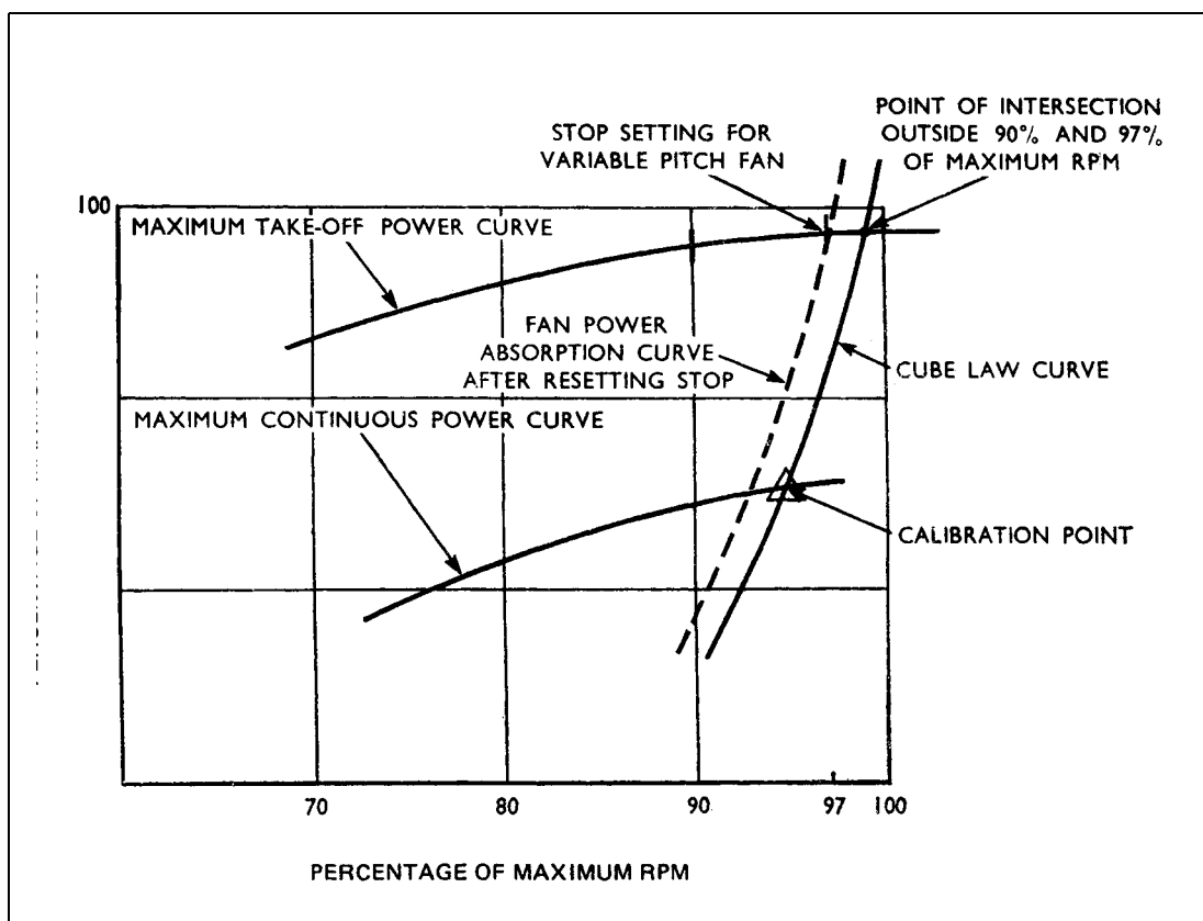
Figure 3 Determination of Type of Test Fan and Pitch Setting Required for a Supercharged Engine
