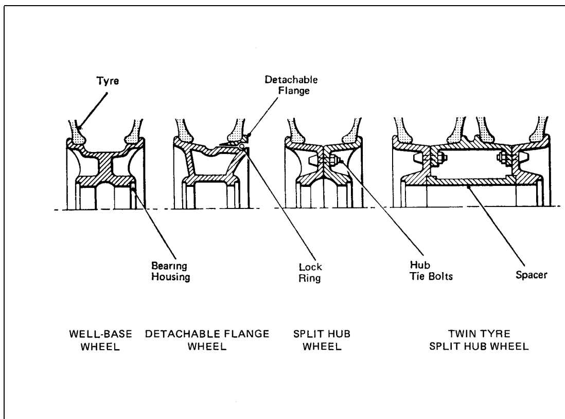
Figure 1 Wheel Types
