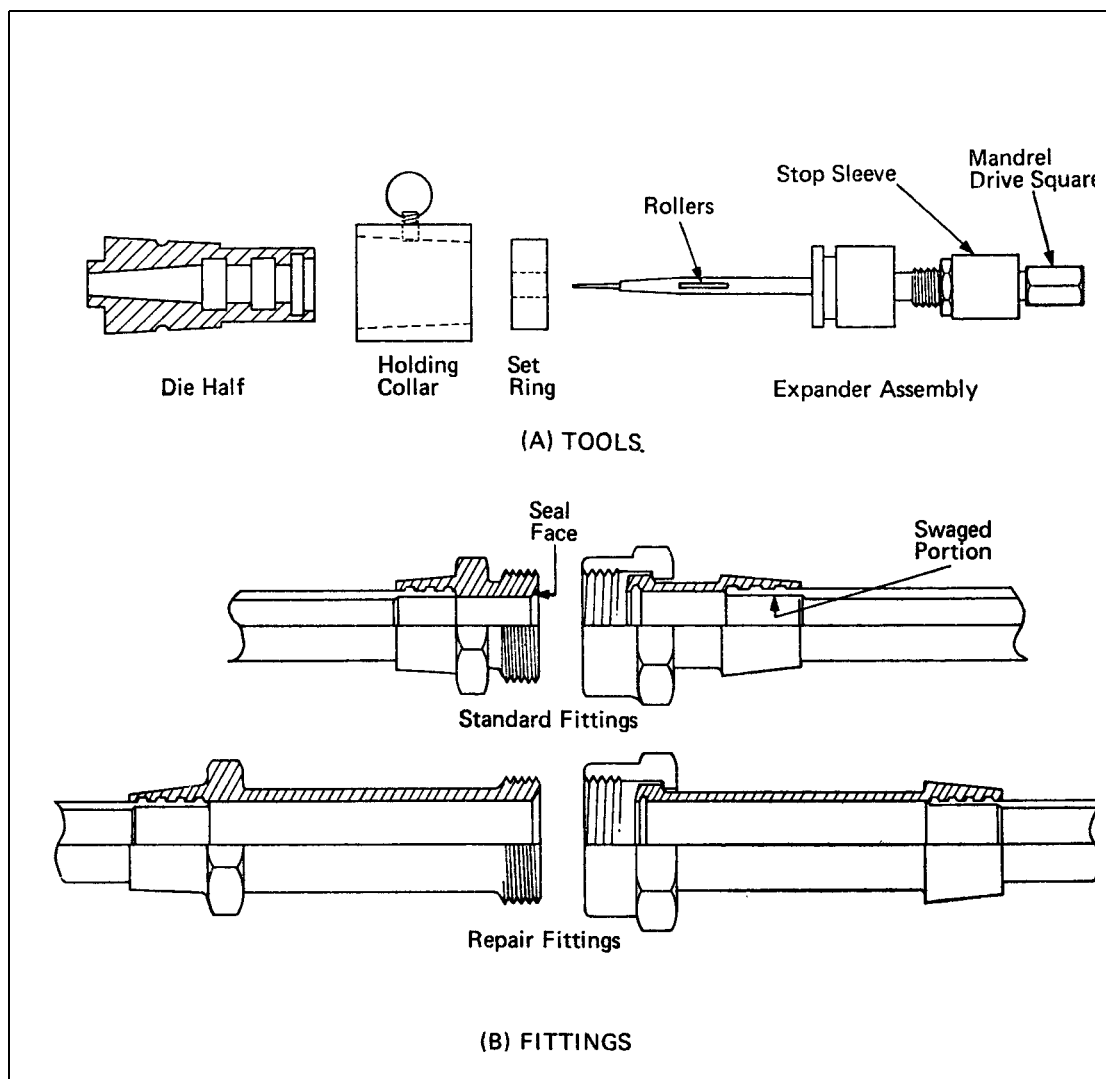
Figure 2 Tools and Typical Repairs for Internal Swaging Process
