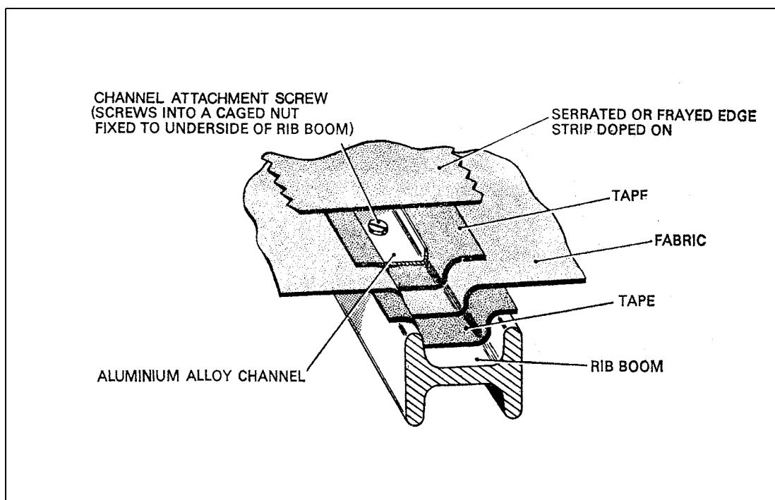
Figure 6 Special Stringing
