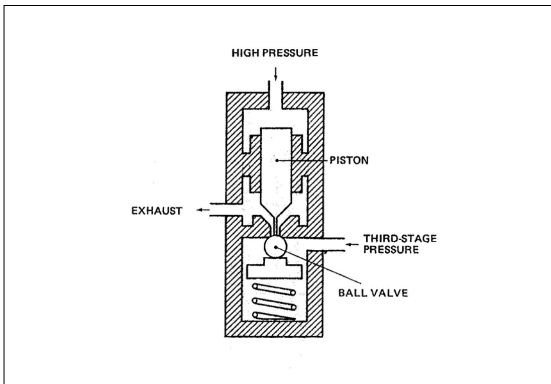
Figure 3 Pressure Regulator
