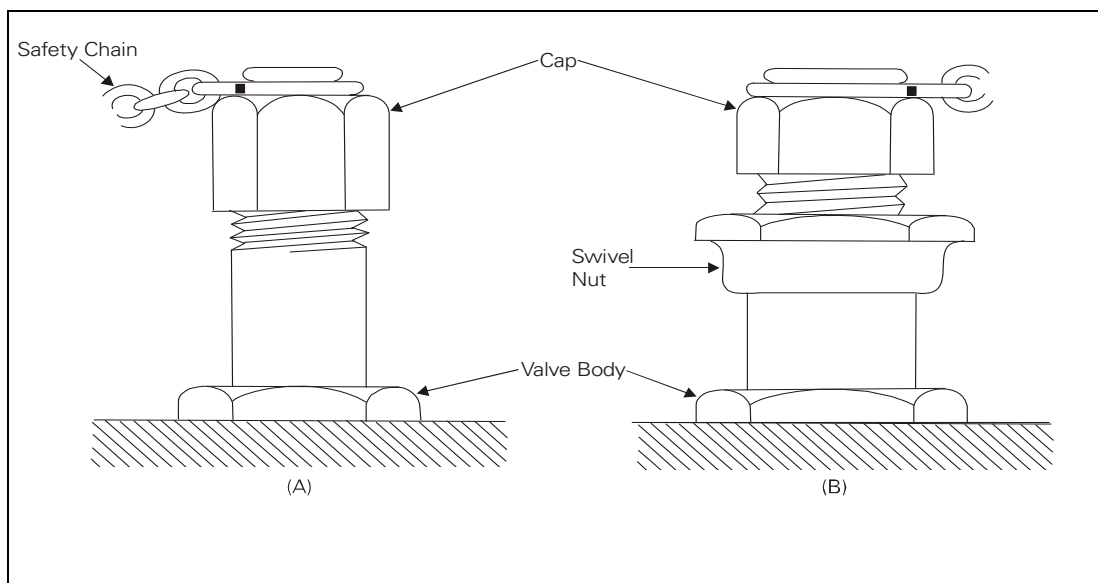
Figure 1 Charging Valves
