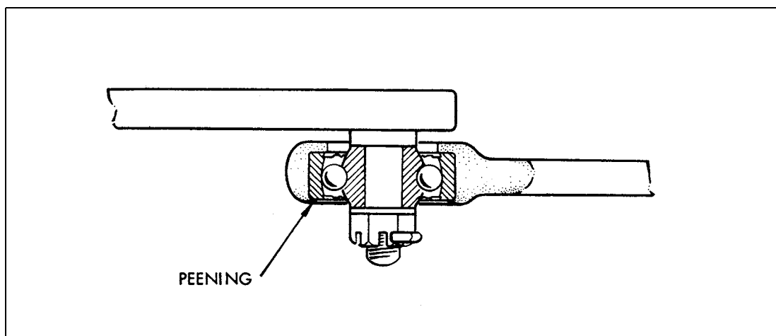
Figure 5 Self-aligning Bearing
