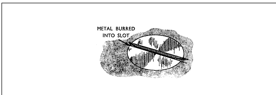
Figure 8 Peening to Lock Countersunk Screws
