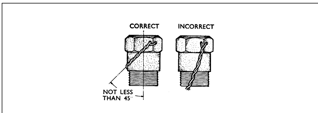
Figure 5 Angle of Approach
