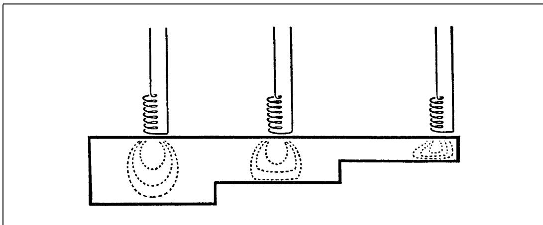
Figure 2 Geometric Effects on Primary Magnetic Field
