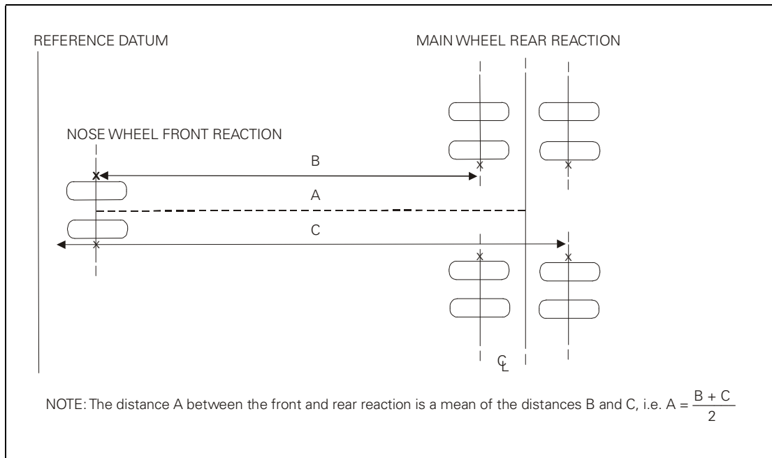
Figure 5 Heavy Aircraft
