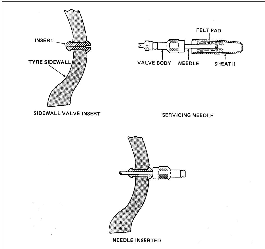
Figure 4 Sidewall Valve
