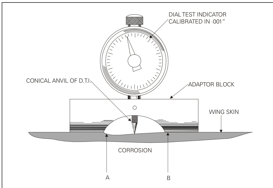
Figure 5 Measurement of Surface Damage
