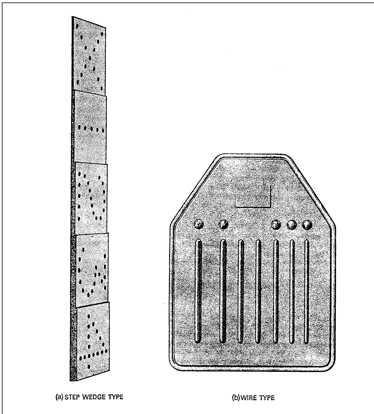
Figure 2 Standard Image Quality Indicators
