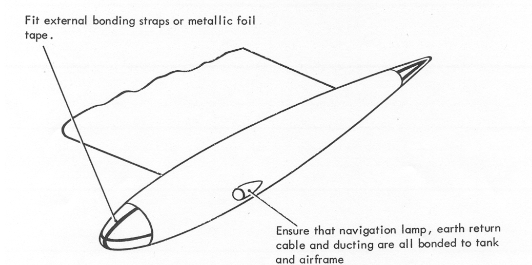
Figure 3 WING TIP TANK (ALL METAL)
