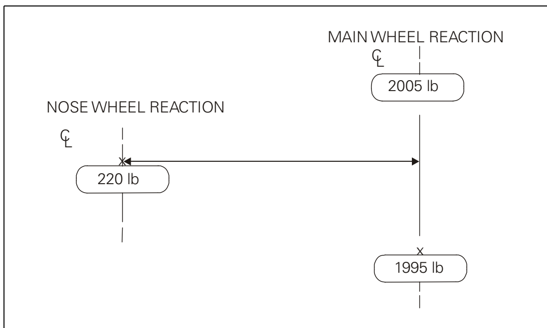
Figure 4 Light Aircraft
