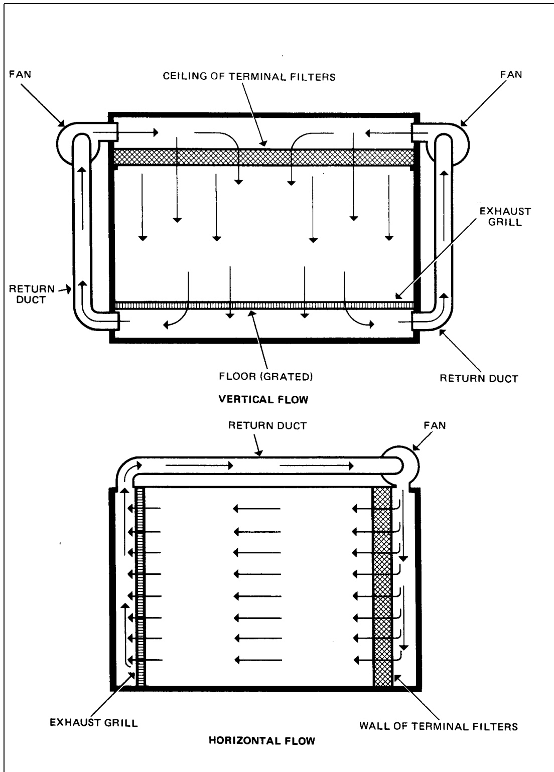
Figure 2 Unidirectional-flow Systems
