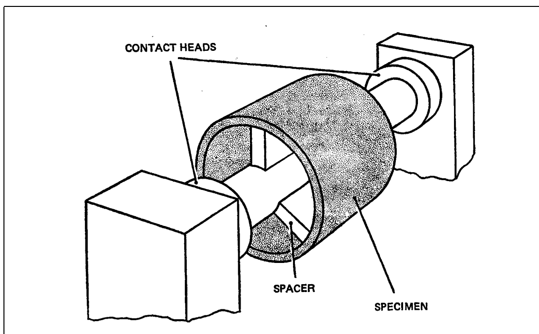
Figure 2 Threading Bar Method
