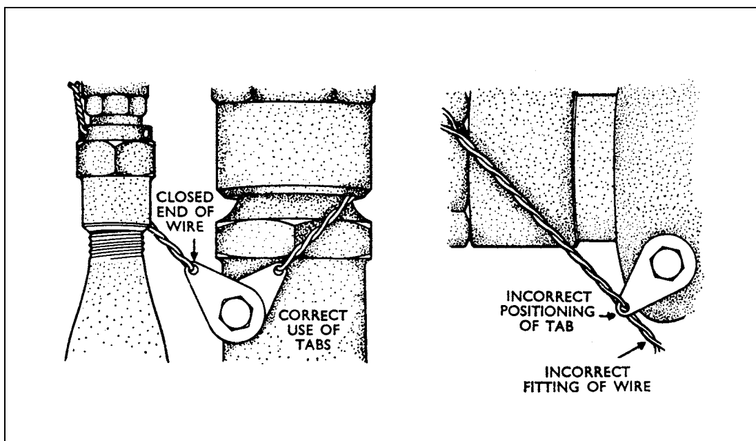
Figure 7 Correct and Incorrect Use of Locking Tabs
