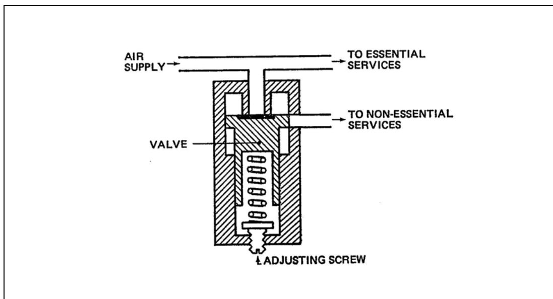
Figure 5 Pressure Maintaining Valve
