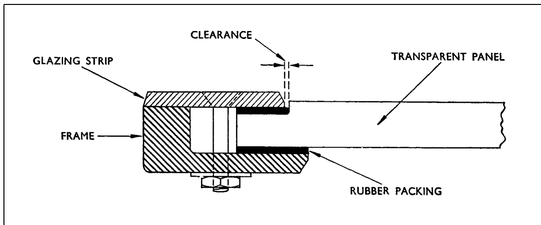
Figure 1 Friction Mounting
