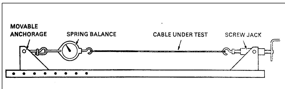
Figure 10 Test Rig for Proof Loading
