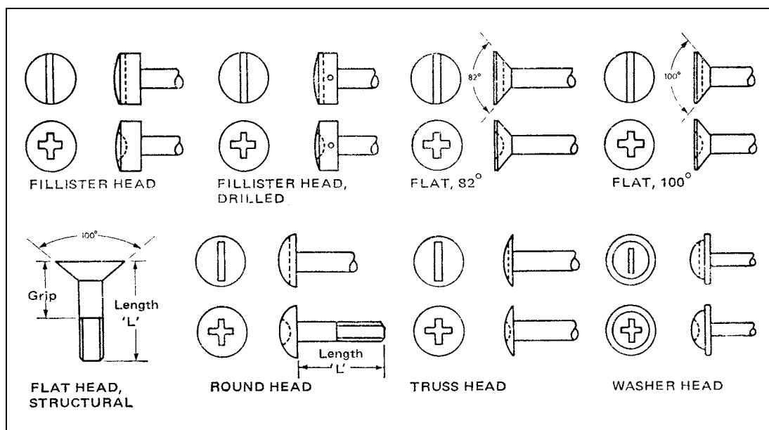
Figure 2 Early Series AN Screws
