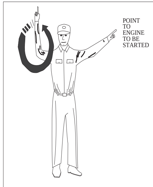
FIG 4-3-12 Start Engine
