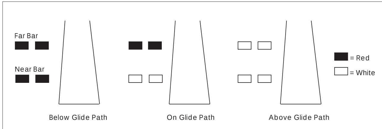
FIG 2-1-2 2-Bar VASI
