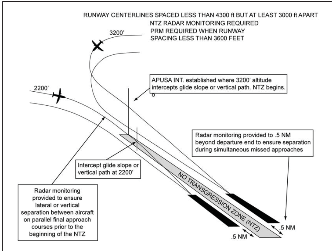
FIG 5-4-22 PRM Approaches (Simultaneous Close Parallel)
