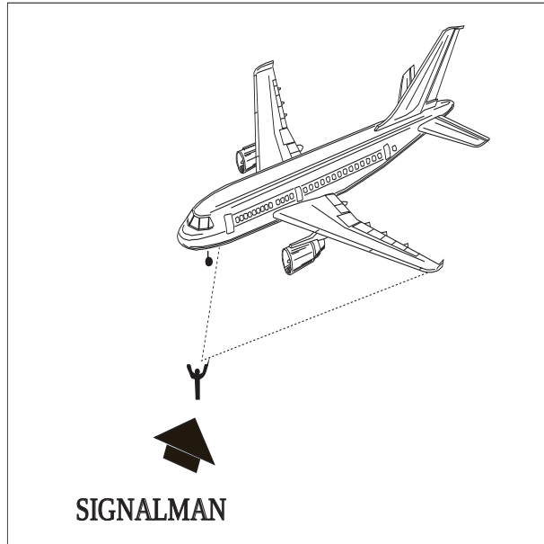
FIG 4-3-10 Signalman's Position
